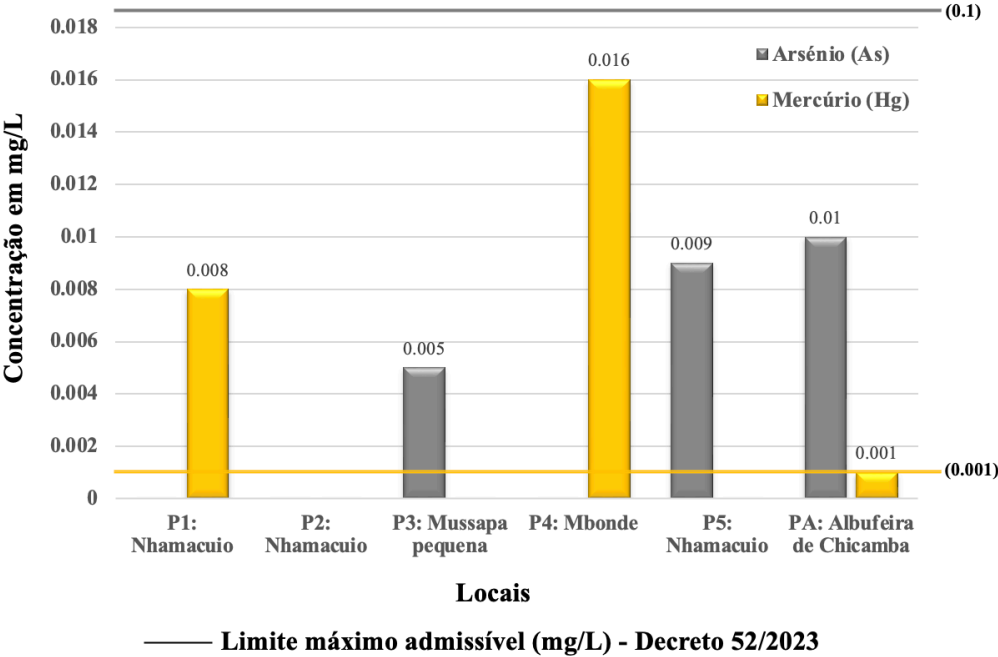
Graph 1: Concentration of heavy metals in mg/L in the water of the Nhamacuio, Mbonde, and Mussapa pequena rivers and in the Chicamba Real reservoir.
